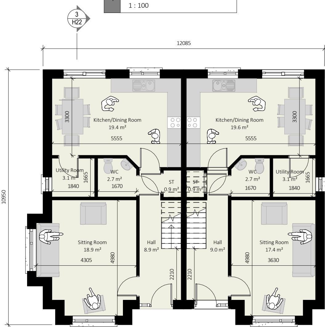
Ground F.F.L 1:100 55.75m 2
