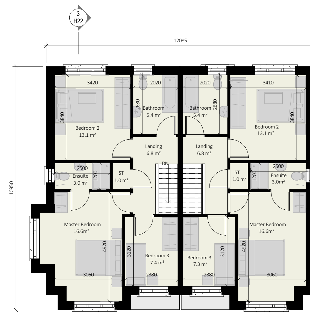
1st Floor F.F.L 1:100 55.75m 2
